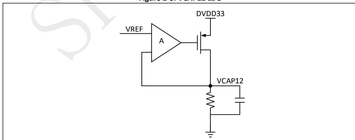
Figure 2-8: VCAP12 LDO
