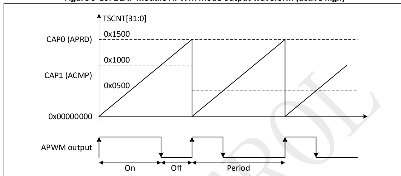
Figure 9-10: ECAP module APWM mode output waveform (active high)
