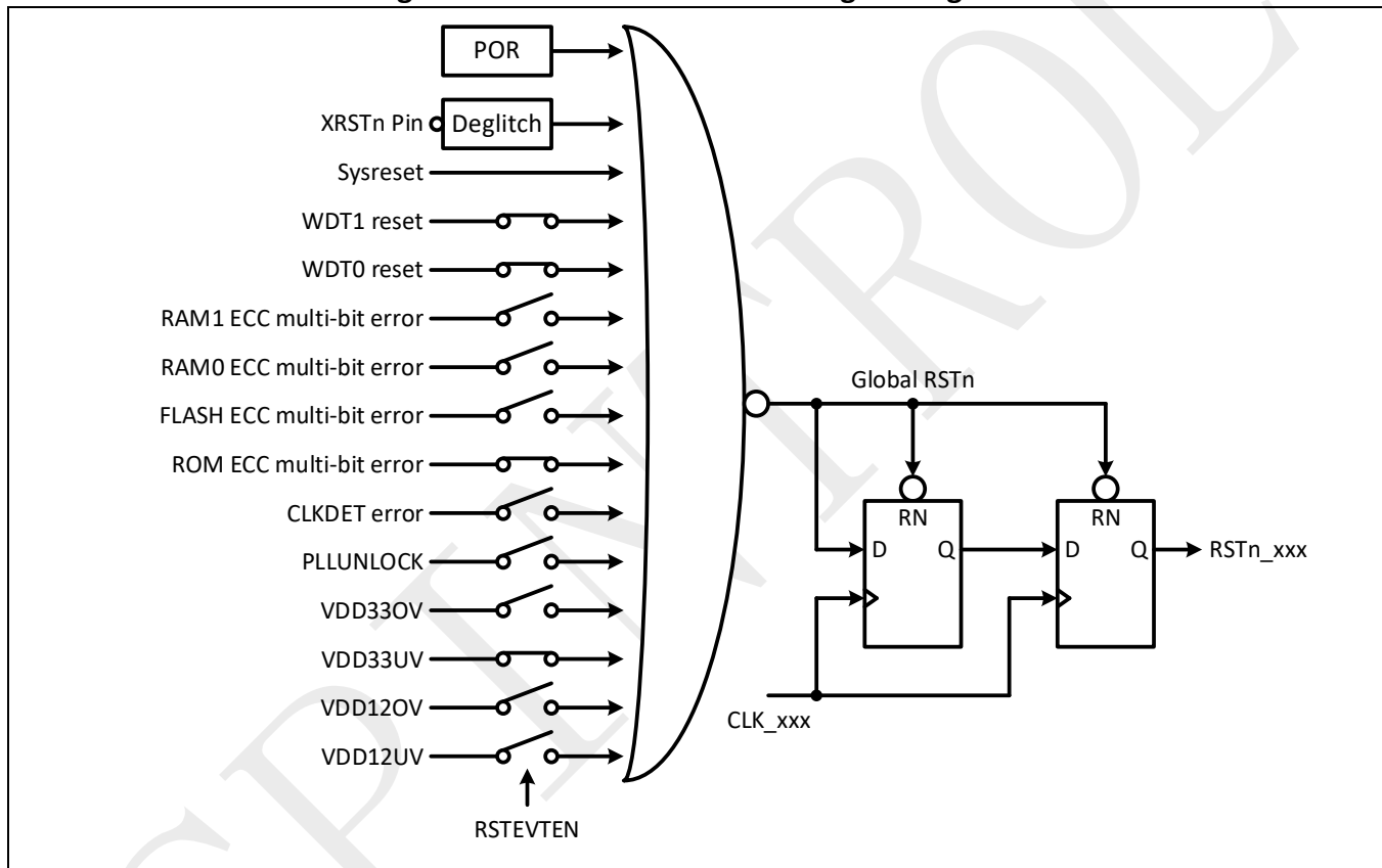
Figure 3-1: Active-low POR reset signal diagram
