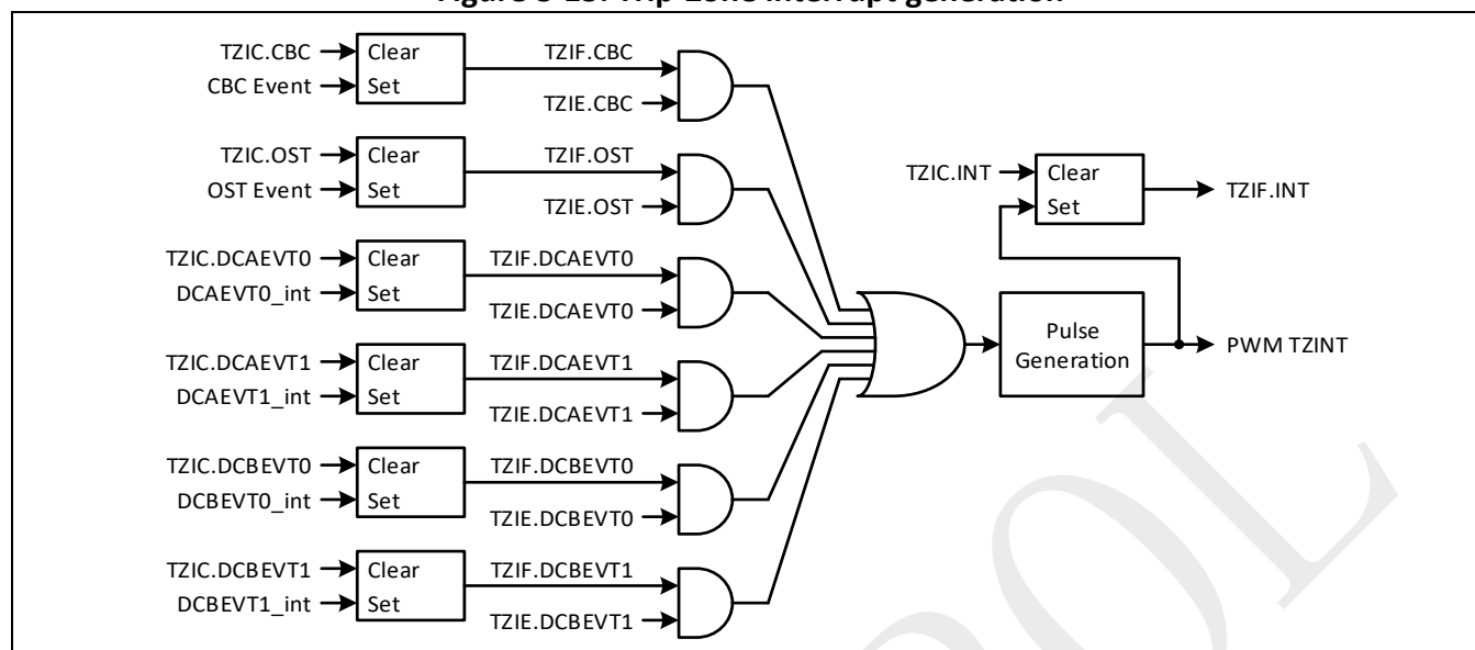
Figure 8-15: Trip-Zone interrupt generation
