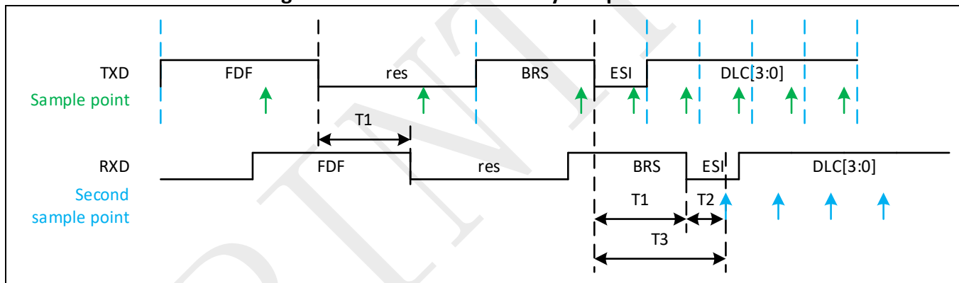
Figure 21-10: Transmitter delay compensation
