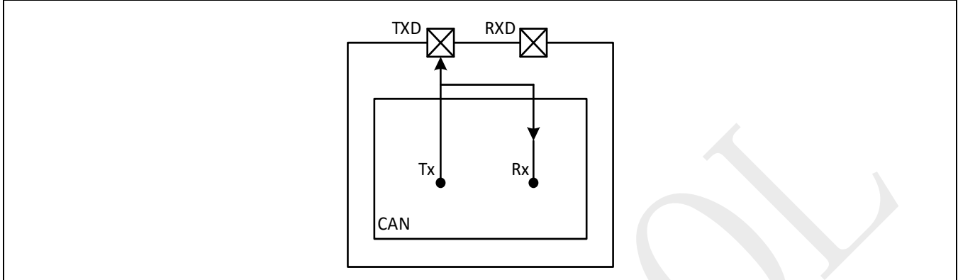
Figure 21-13: External loopback mode
