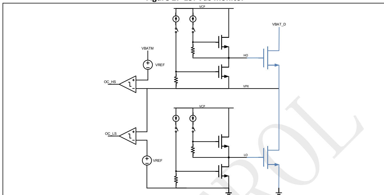
Figure 27-15: Vds monitor
