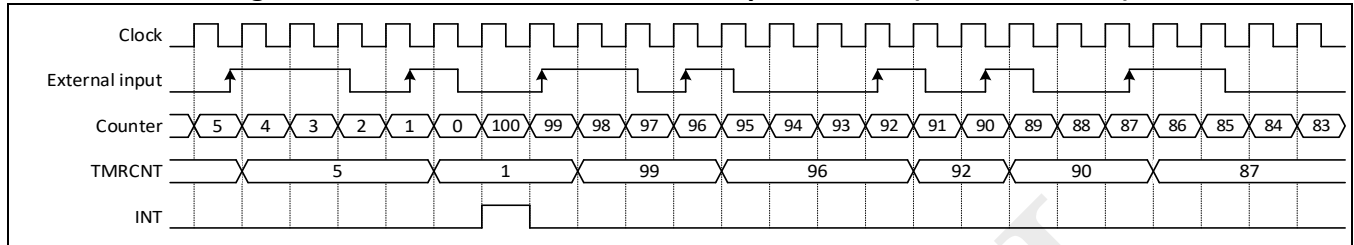
Figure 6-5: Timer waveform in event capture mode (TMRLOAD=100)
