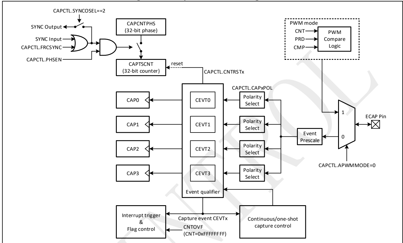
Figure 9-3: Capture function diagram
