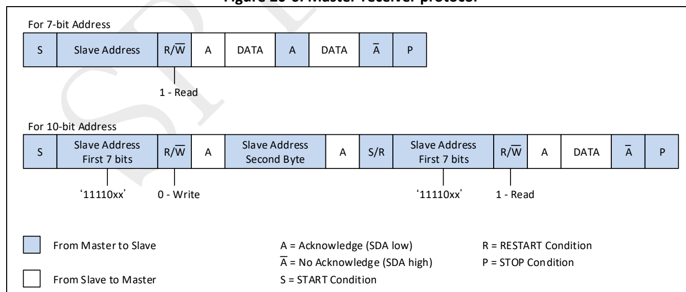
Figure 20-6: Master-receiver protocol
