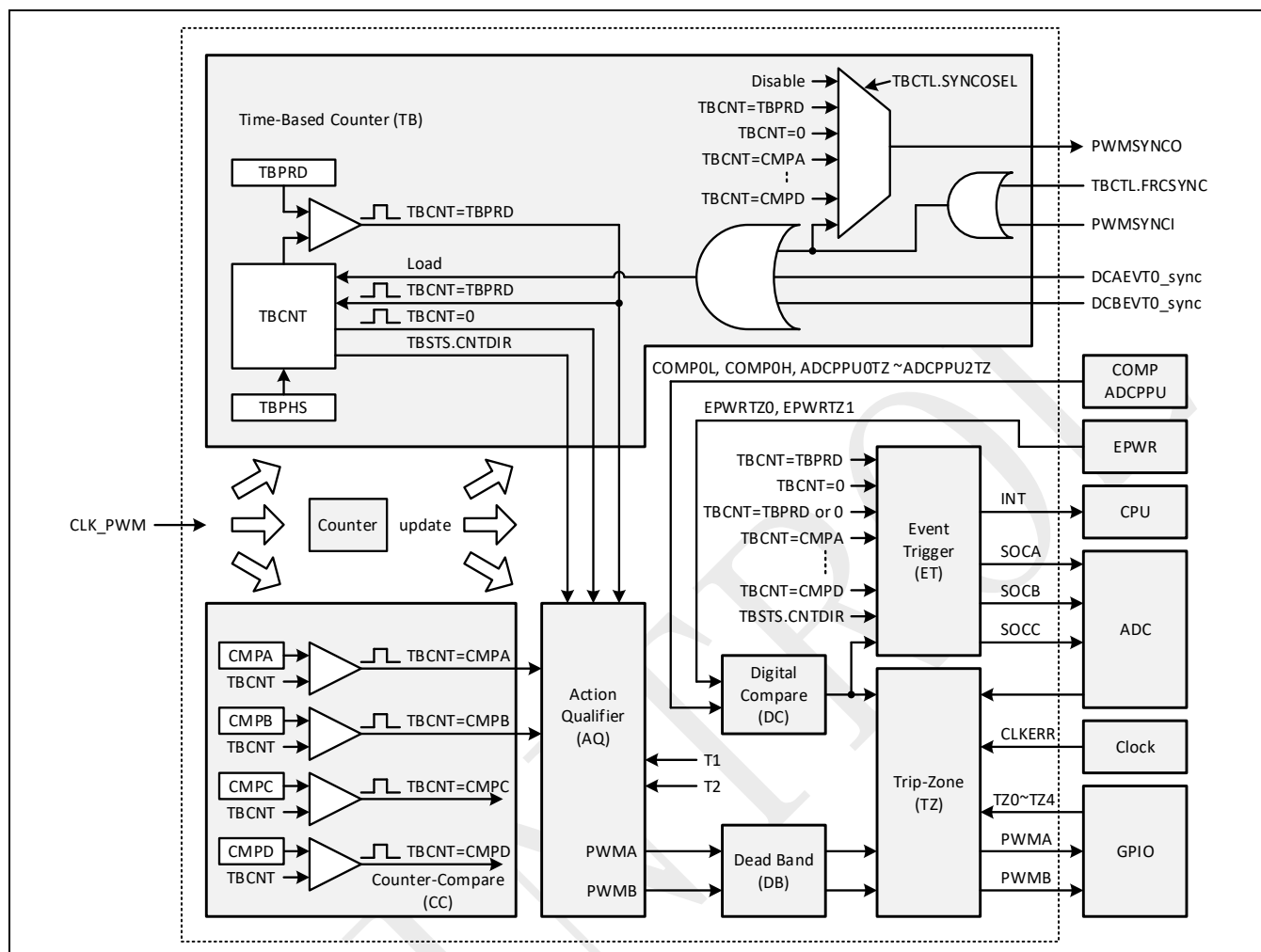
Figure 8-2: PWM architecture
