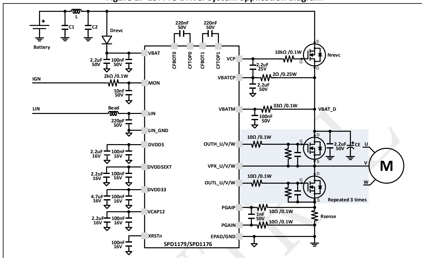
Figure 27-19: Pre-Driver system application diagram
