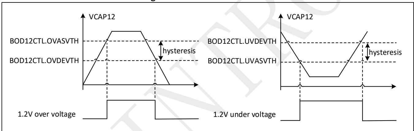
Figure 2-13: VCAP12 thresholds
