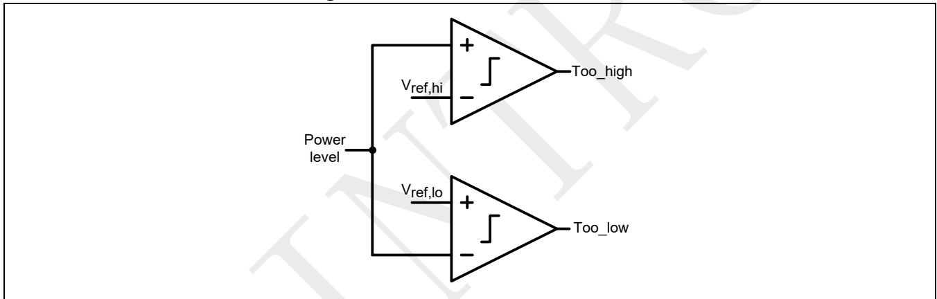
Figure 27-3: Basic structure of BOD
