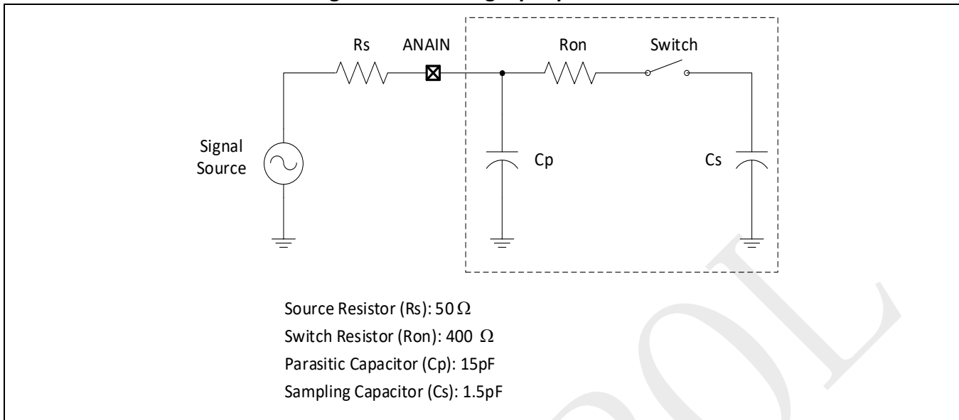
Figure 10-3: Analog input pin model
