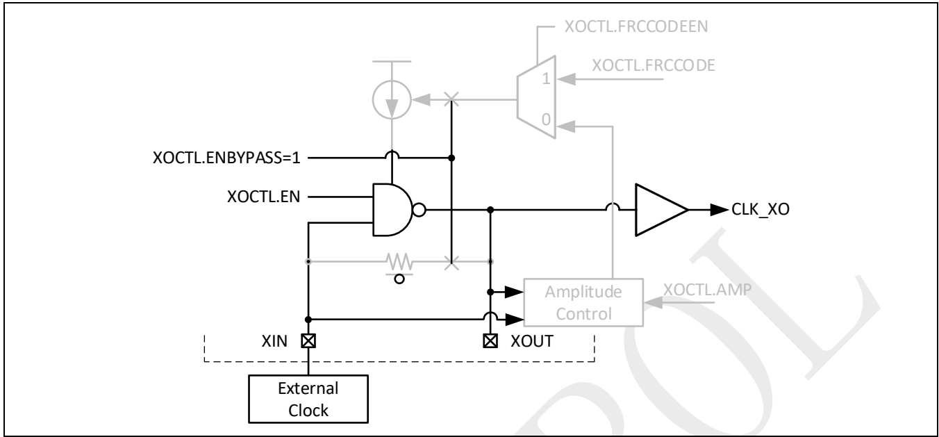
Figure 3-5: External clock
