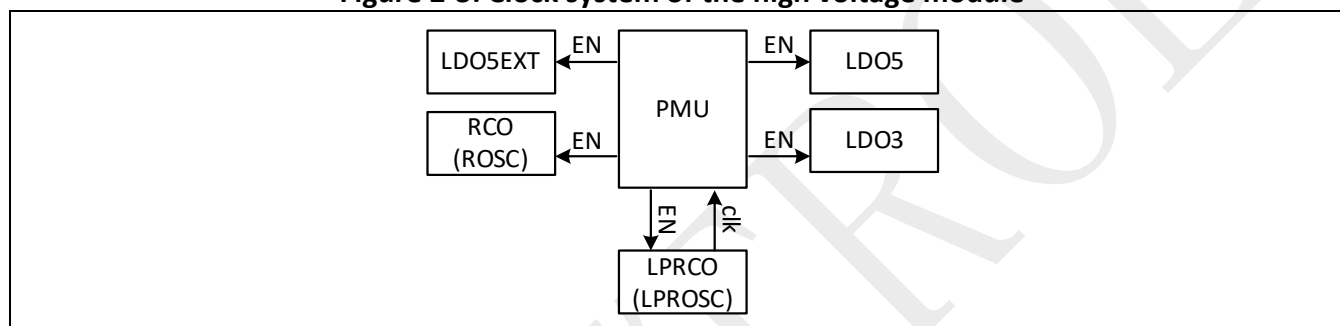
Figure 2-3: Clock system of the high voltage module
