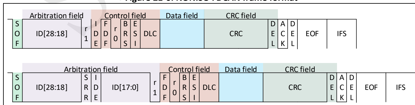
Figure 21-6: NONISO FDCAN frame format
