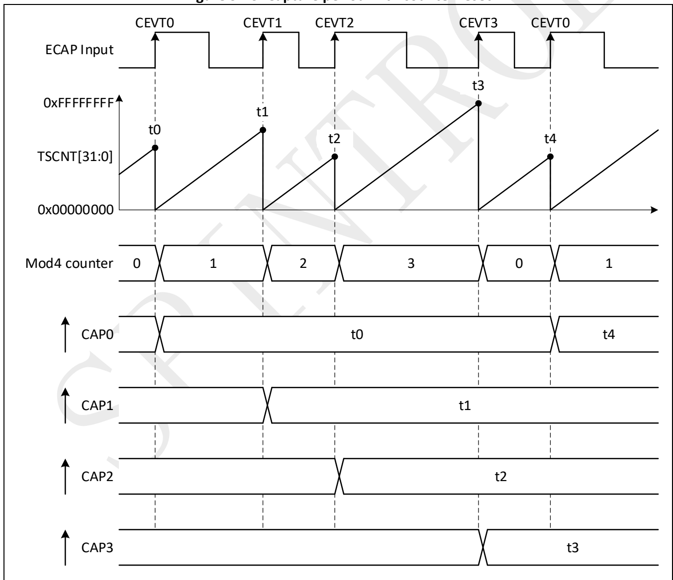
Figure 9-13: Capture period with counter reset
