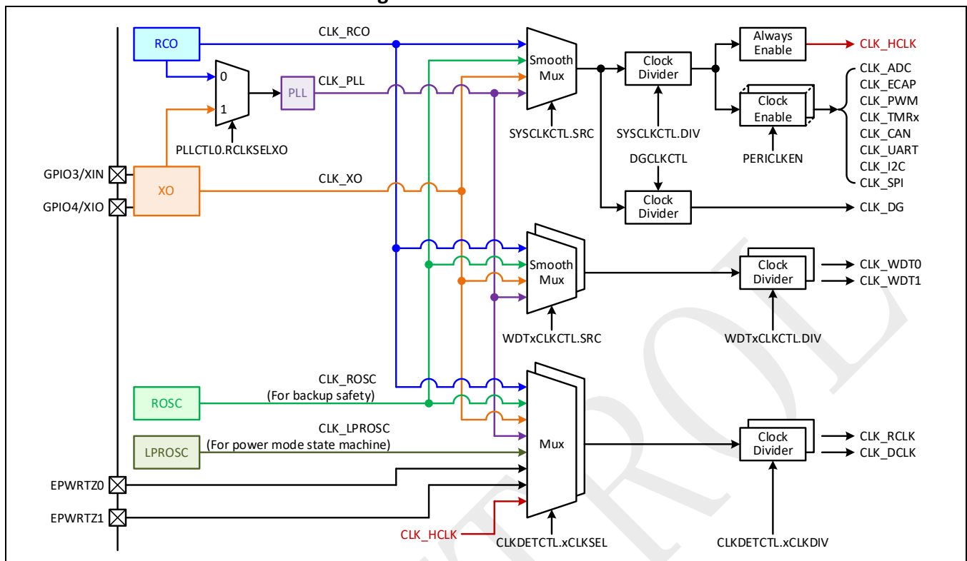
Figure 3-3: Clock overview
