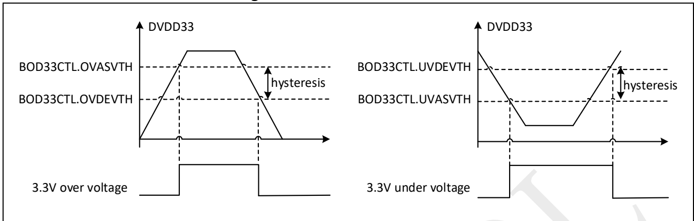
Figure 2-12: DVDD33 thresholds
