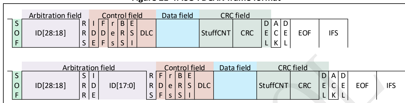
Figure 21-4: ISO FDCAN frame format
