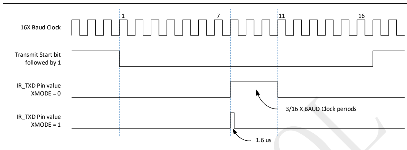
Figure 18-8: XMODE example
