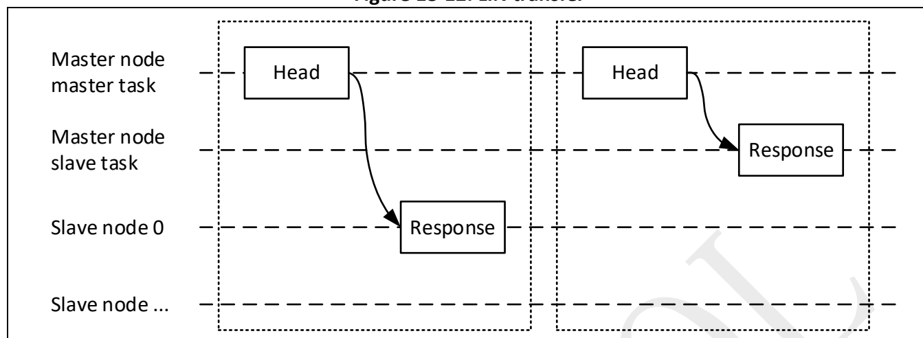
Figure 18-12: LIN transfer
