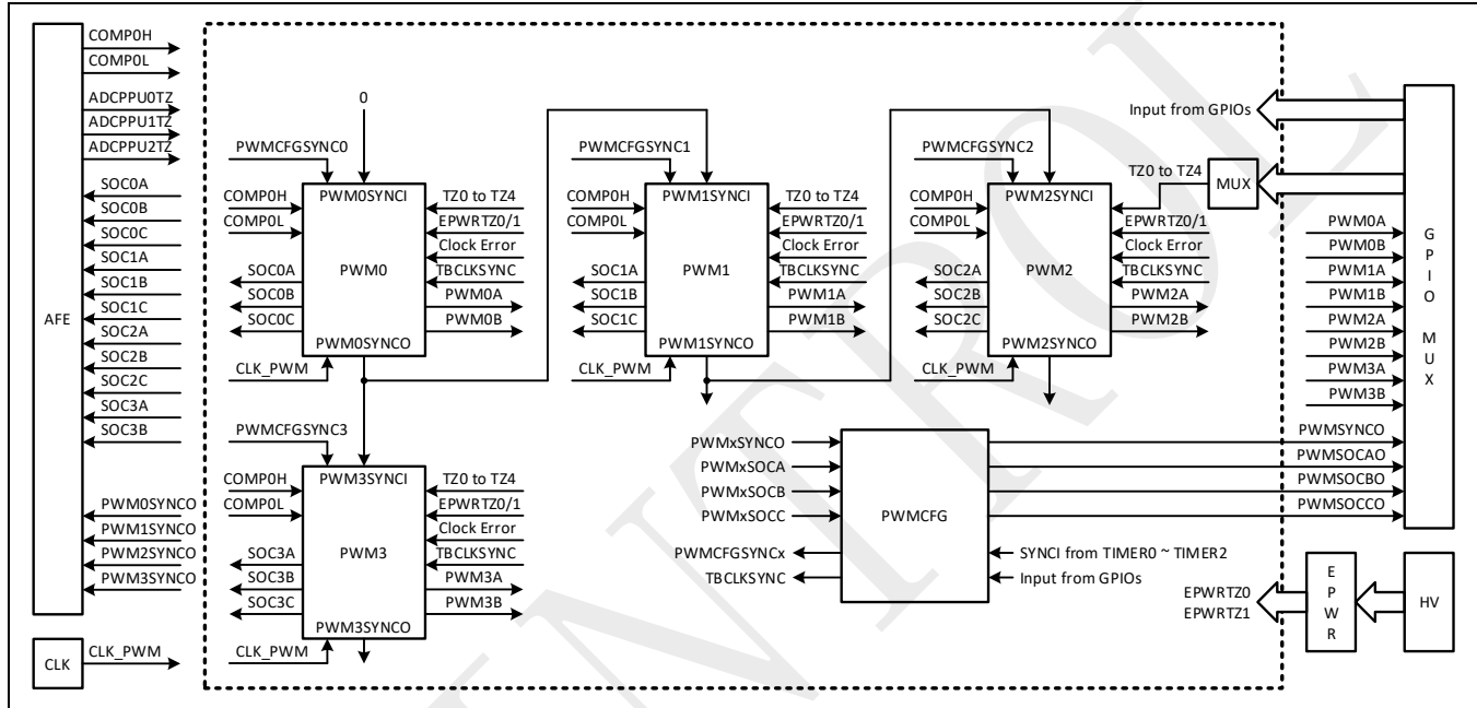
Figure 8-1: PWM overview
