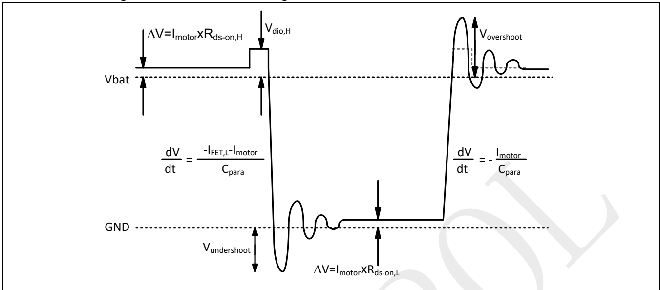
Figure 27-11: VPX switching in case of current delivered to the driver
