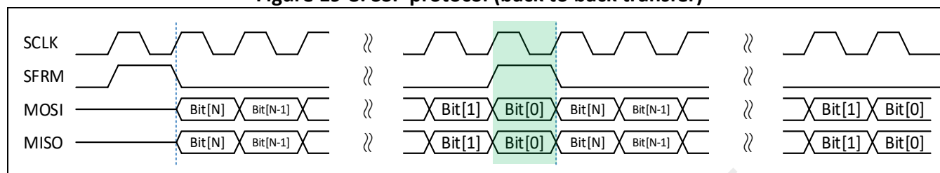
Figure 19-8: SSP protocol (back to back transfer)
