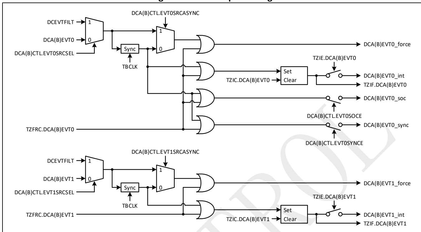
Figure 8-19: Event processing
