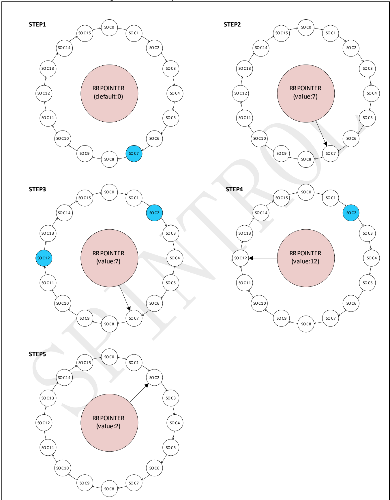
Figure 10-6: Example for round robin arbitration
