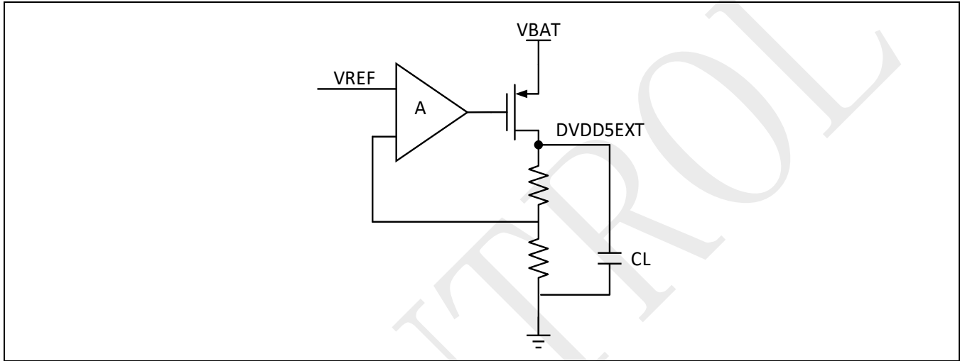
Figure 2-9: DVDD5EXT LDO
