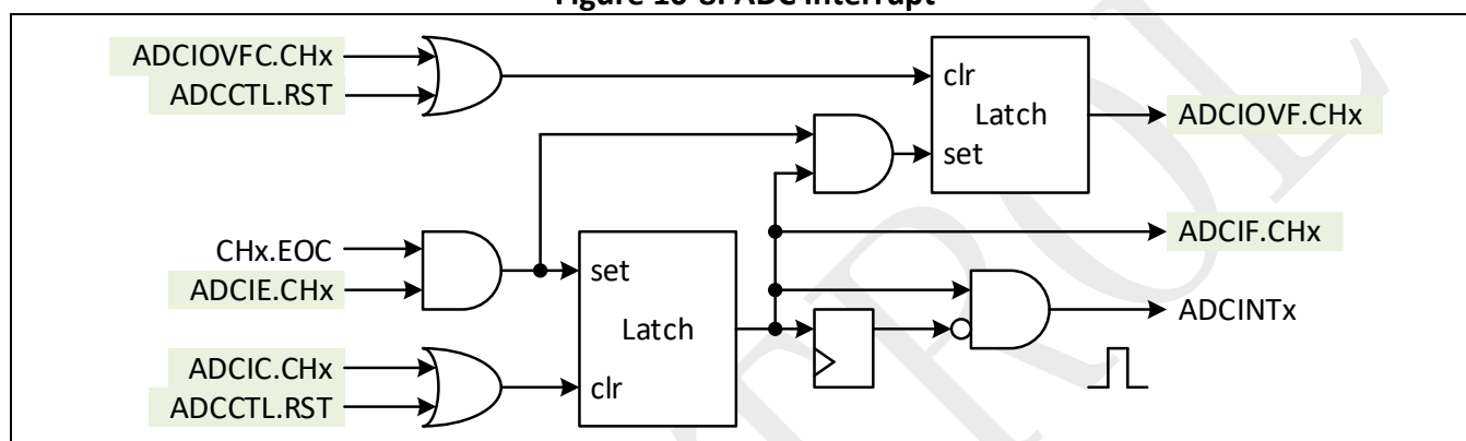
Figure 10-8: ADC Interrupt
