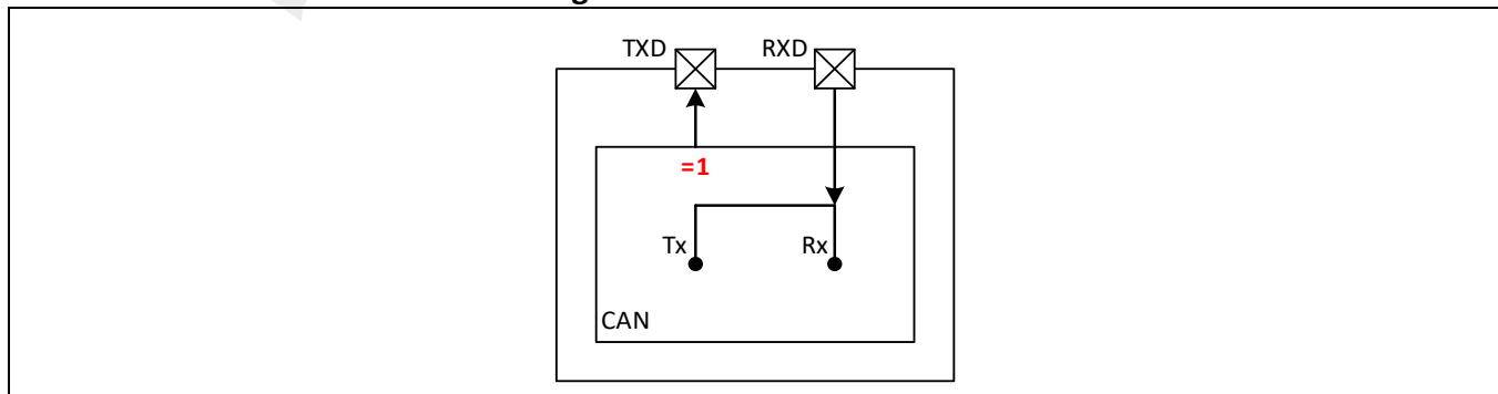
Figure 21-11: Monitor mode
