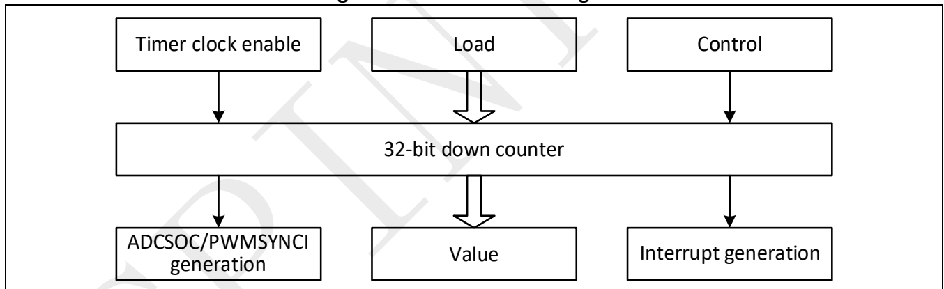
Figure 6-6: GPT run flow diagram
