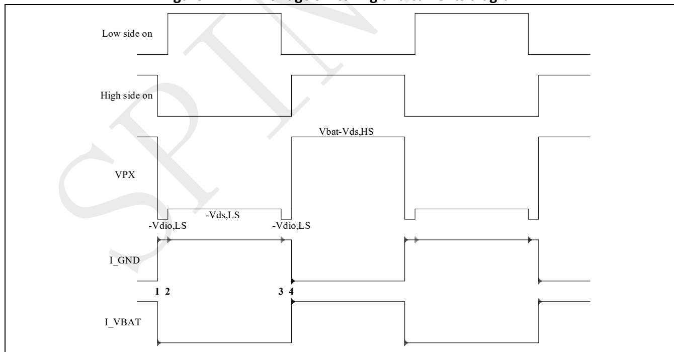
Figure 27-14: H-bridge switching and currents diagram
