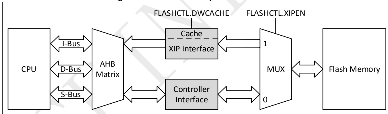
Figure 23-1: Flash memory access interfaces
