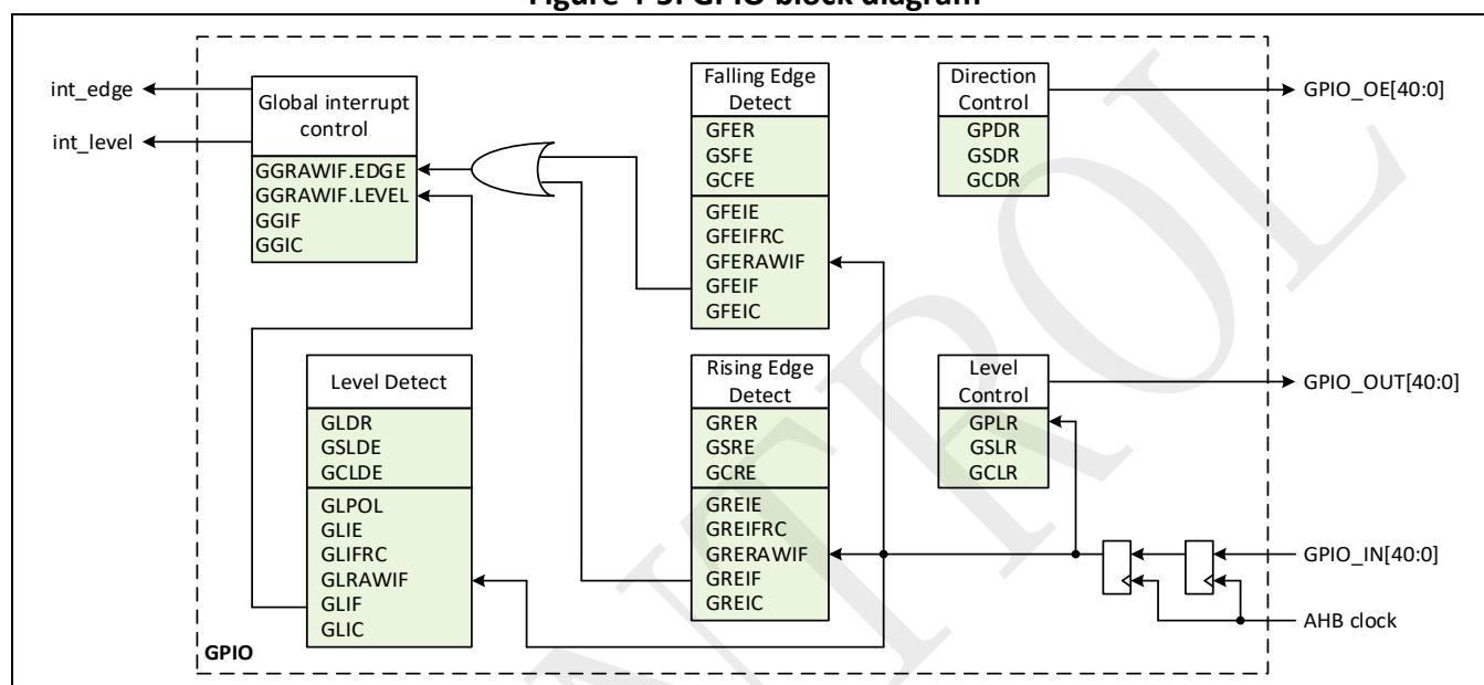
Figure 4-5: GPIO block diagram
