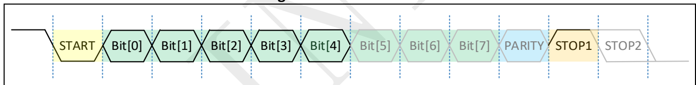
Figure 18-4: UART frame
