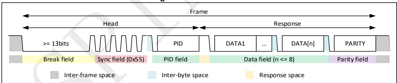
Figure 18-11: LIN frame
