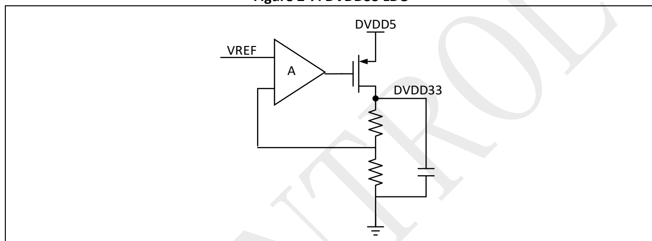
Figure 2-7: DVDD33 LDO
