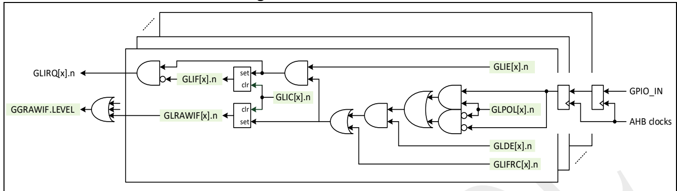
Figure 4-8: GPIO level detect
