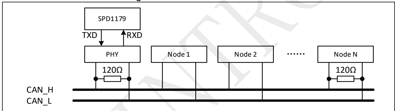
Figure 21-2: CAN device connection
