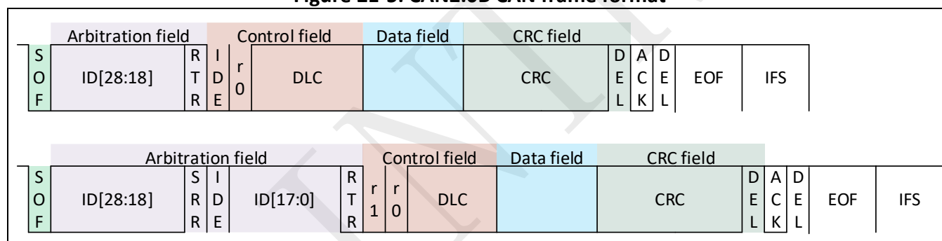
Figure 21-5: CAN2.0B CAN frame format
