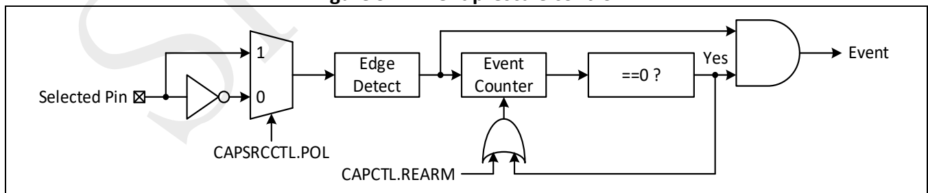
Figure 9-4: Event prescale control
