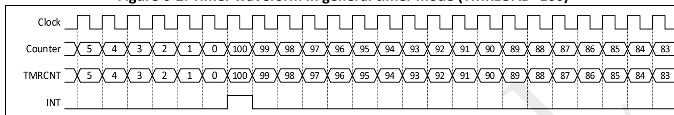
Figure 6-2: Timer waveform in general timer mode (TMRLOAD=100)
