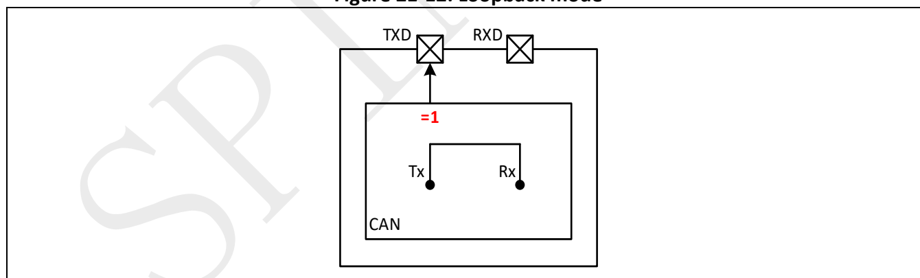
Figure 21-12: Loopback mode
