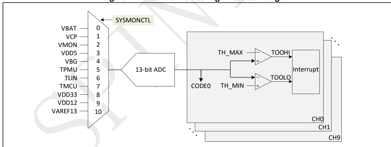
Figure 11-1: 13-bit Monitoring ADC block diagram
