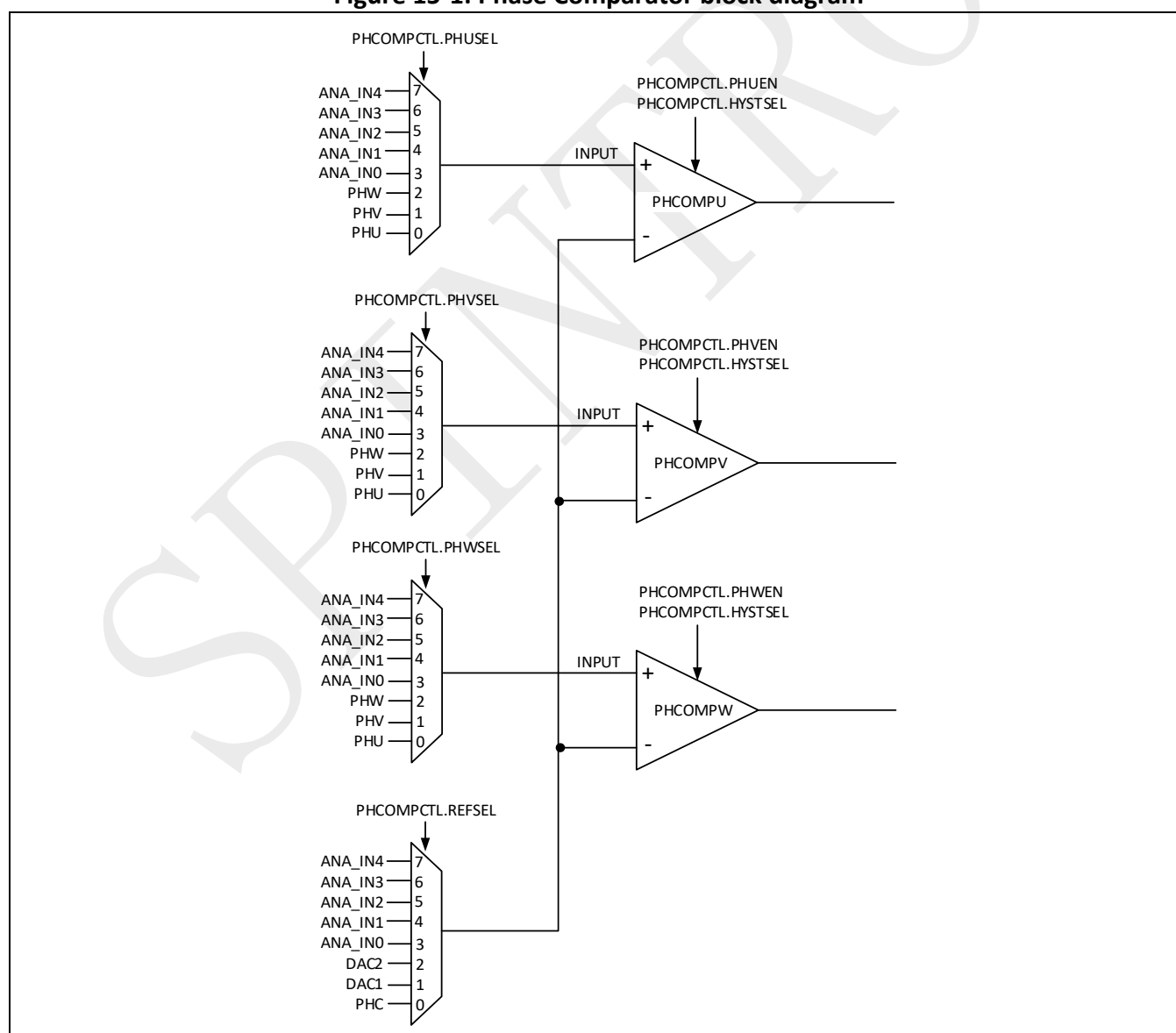
Figure 15-1: Phase Comparator block diagram
