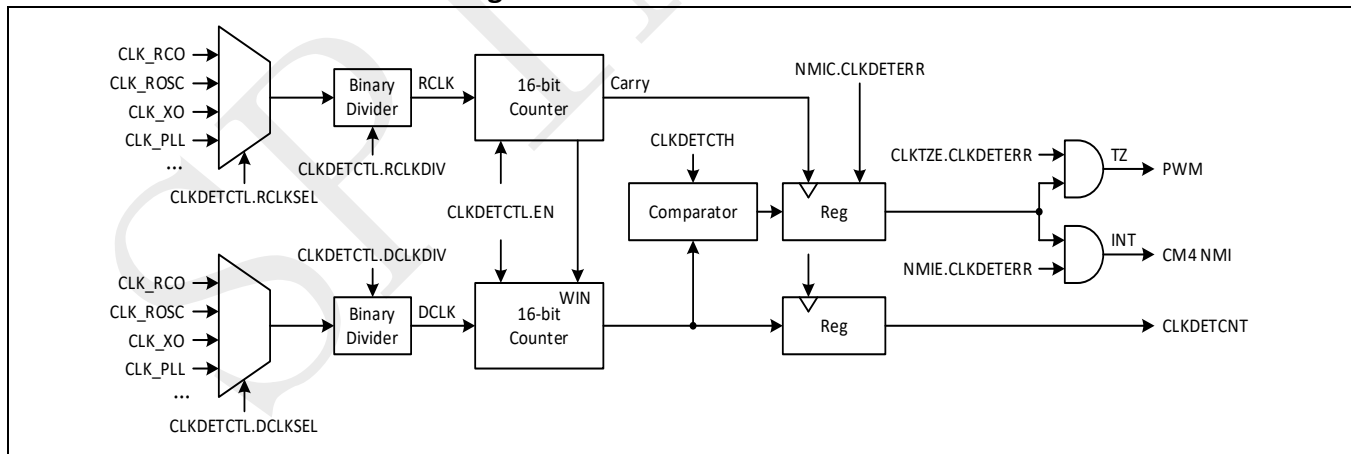
Figure 3-8: Clock cross-detection
