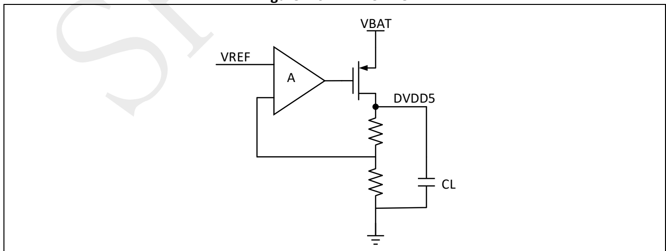
Figure 2-6: DVDD5 LDO
