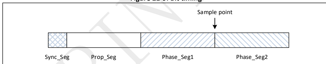
Figure 21-9: Bit timing
