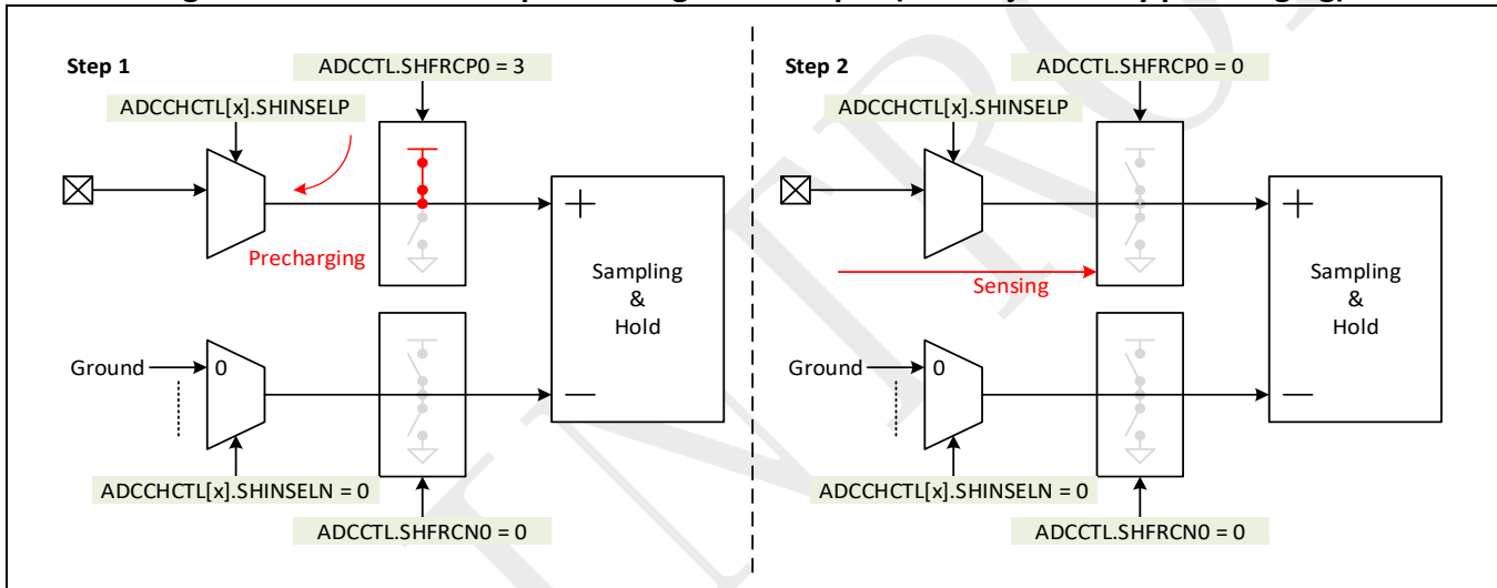
Figure 10-11: Detect the pin floating of ADC input (fault injection by precharging)
