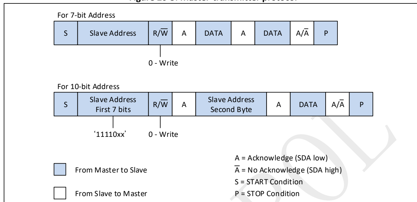
Figure 20-5: Master-transmitter protocol
