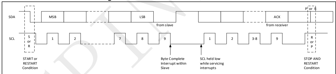
Figure 20-1: Data transfer on the I2C bus
